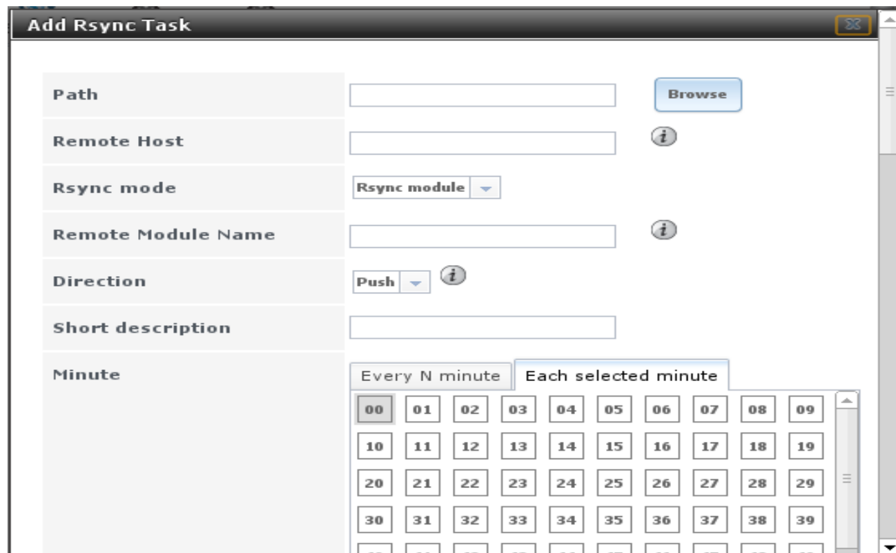
Figure 4.4a: Adding an Rsync Task
