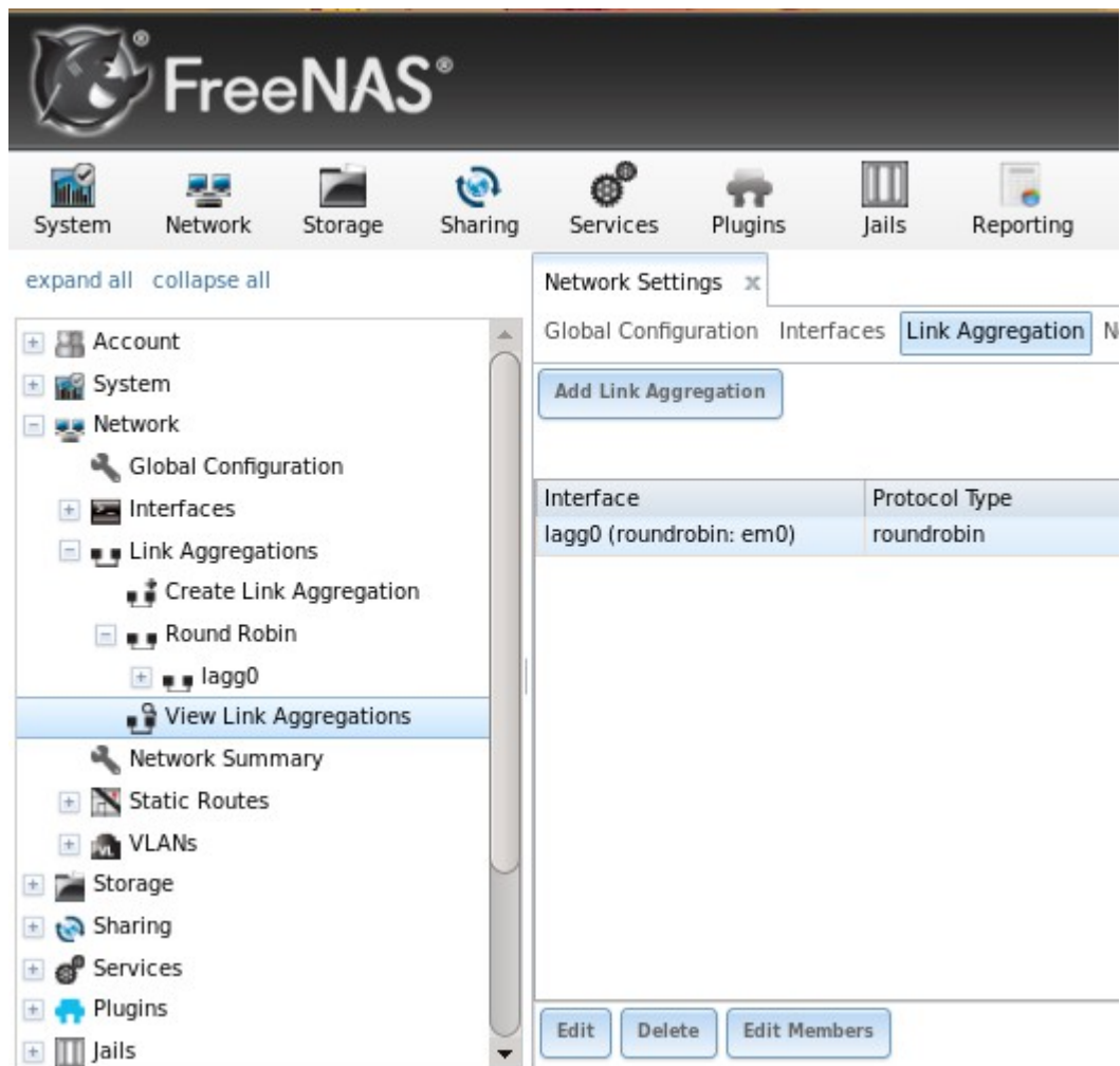
Figure 5.3b: Viewing Link Aggregations
