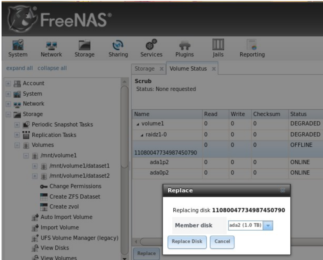
Figure 6.3r: Replacing a Failed Disk
