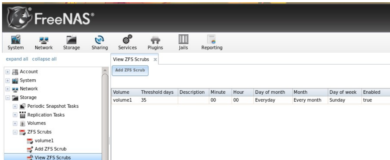
Figure 6.4a: Viewing a Volume's Default Scrub Settings
