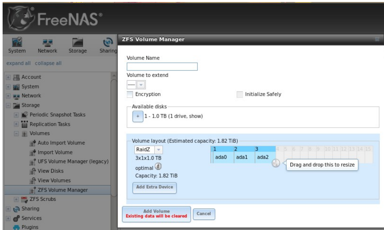
Figure 6.3f: Creating a ZFS Pool Using Volume Manager
