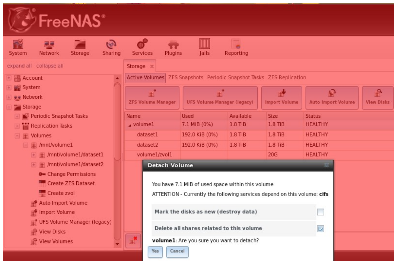
Figure 6.31: Detaching or Deleting a Volume
