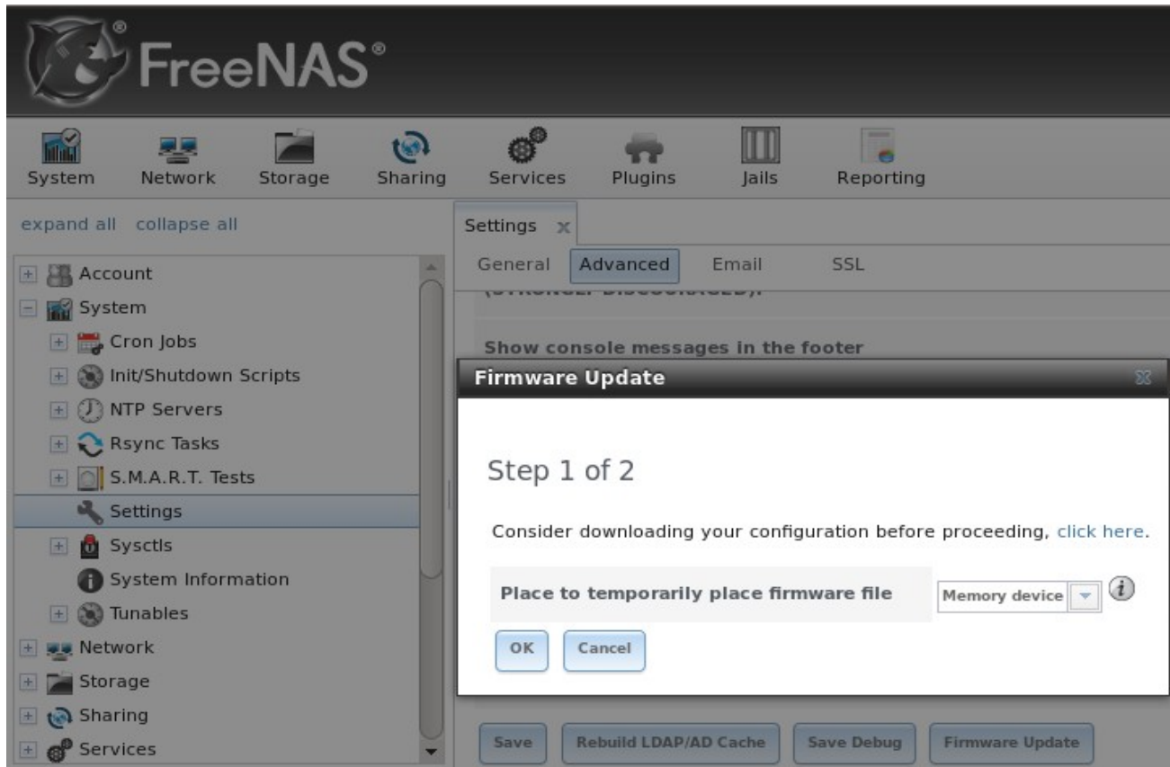
Figure 2.6d: Upgrading FreeNAS® From the GUI
