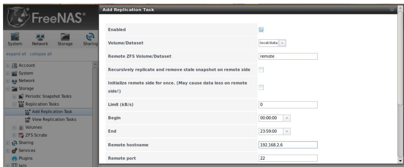
Figure 6.2b: Adding a Replication Task
