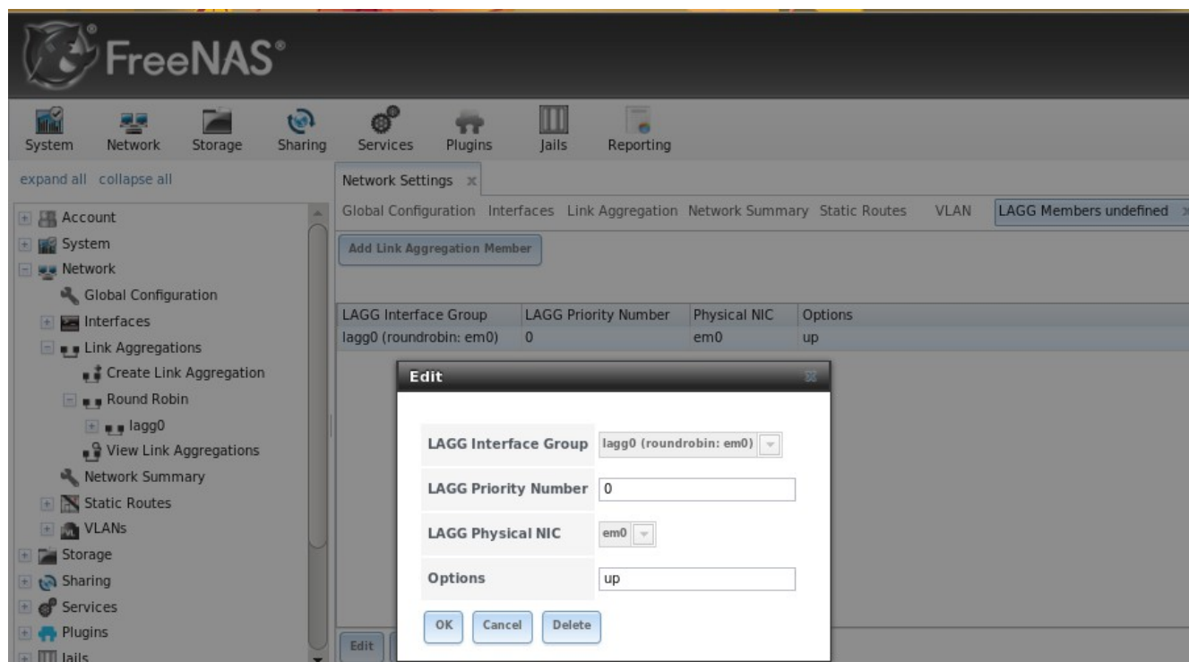
Figure 5.3d: Editing a Member Interface
