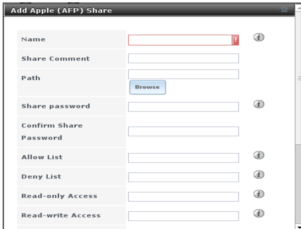
Figure 7.1a: Creating an AFP Share
