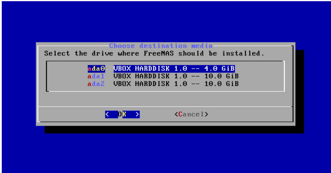
Figure 2.3b: Selecting Which Drive to Install Into
