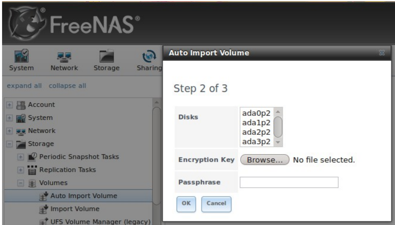
Figure 6.3c: Decrypting the Disks Before Importing the ZFS Pool
