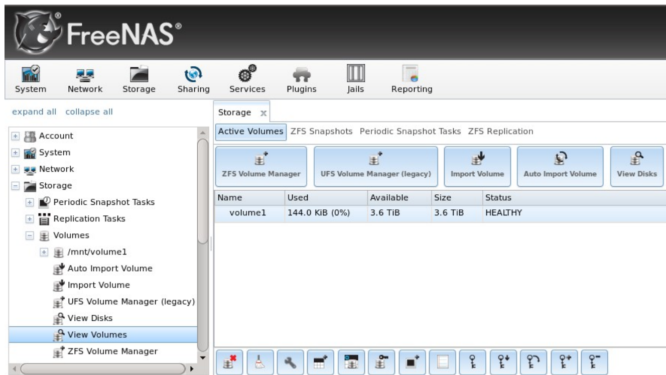
Figure 6.3o: Encryption Icons Associated with an Encrypted ZFS Volume
