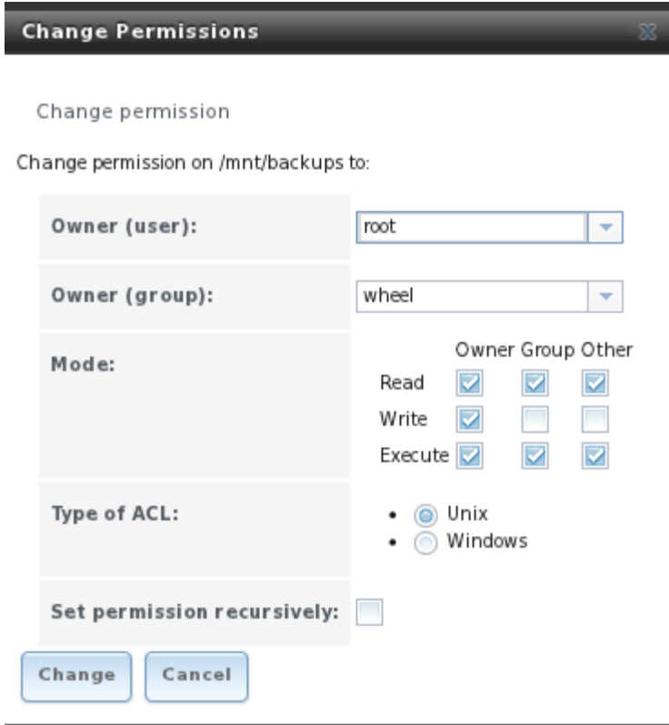
Figure 6.3p: Changing Permissions on a Volume or Dataset
