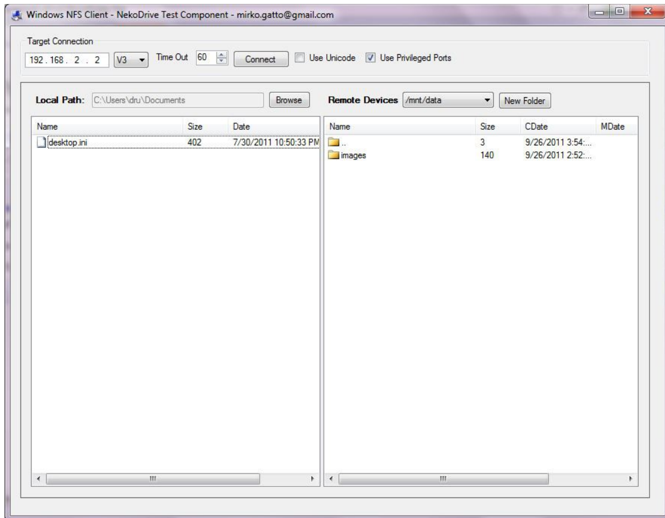
Figure 7.2b: Using the NekoDrive NFSClient from Windows 7 Home Edition
