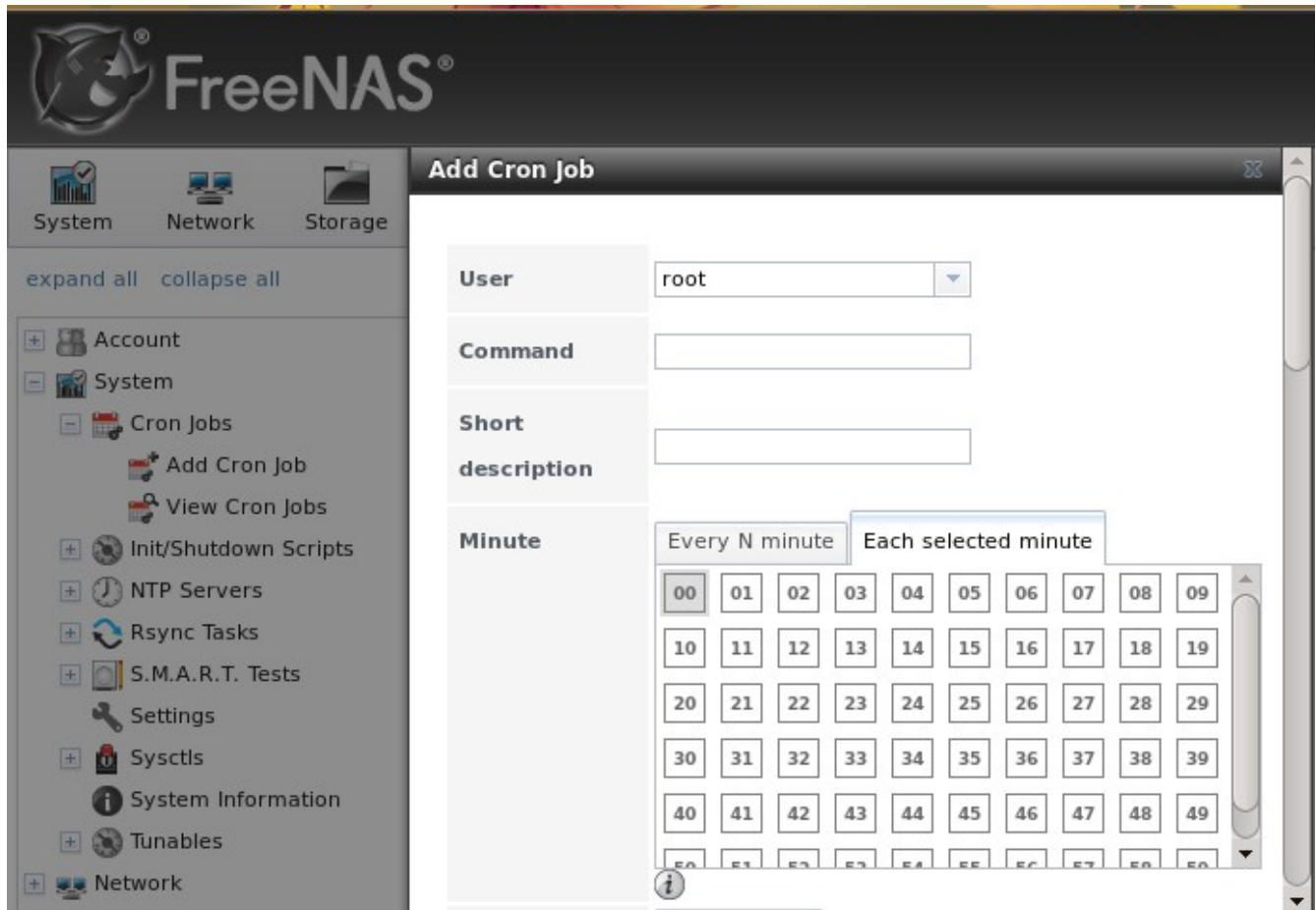
Figure 4.1a: Creating a Cron Job
